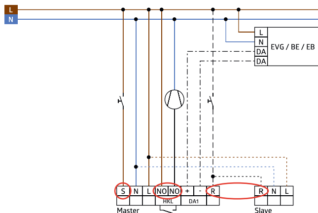
DALI-DSI HVAC/HKL BROADCAST
